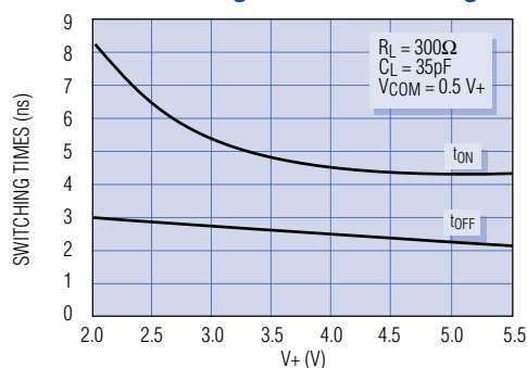
Switching Time vs. Voltage
